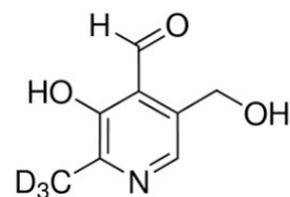
Pyridoxal-(methyl-d3)
